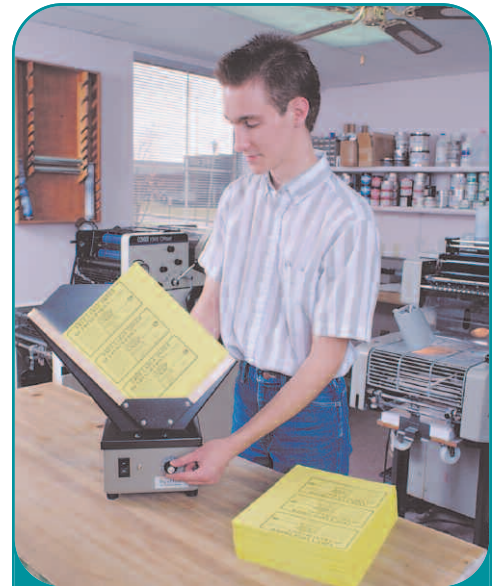
Easily adjustable vibration is available on all Syntron® joggers. Popular with printers using offset presses or duplicating machines, the Model J-1 single bin, shown here, is perfect for aerating and aligning reams of tightly packed paper providing smooth, reliable feeding.
