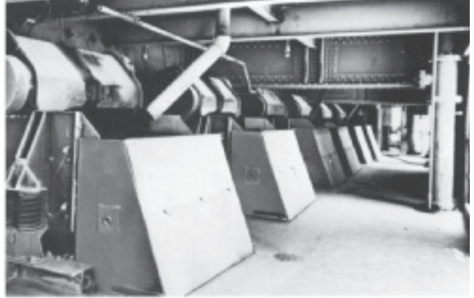
Twelve Link-Belt® Model SG2512 vibrating screens size limestone at a rate of 4,200 tons per hour.
