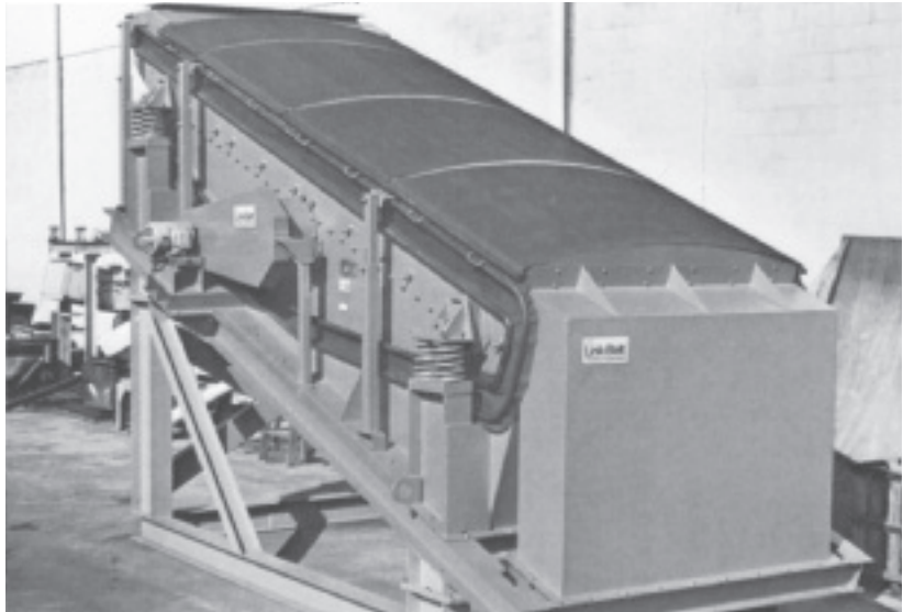
Model CS 1616 with trelleborg rubber enclosure.
