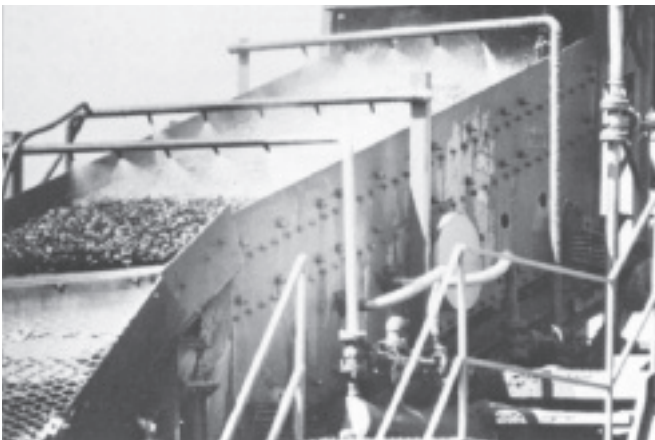
Link-Belt® Model CS-3616 Vibrating Screen handling crushed stone in a quarry.
