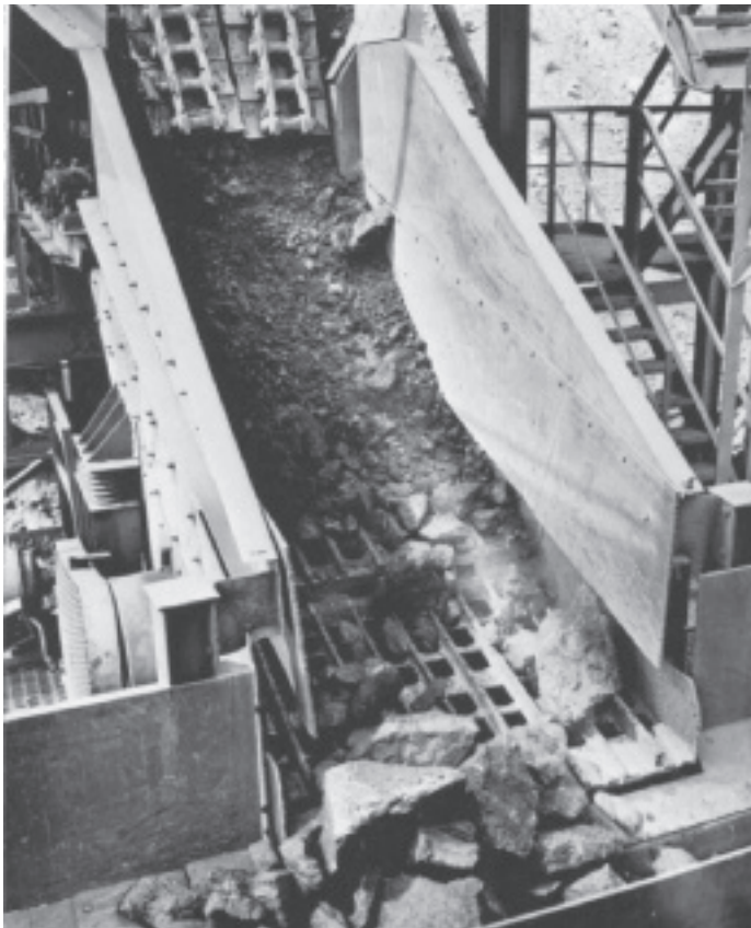
Link-Belt® Model BA heavy duty vibrating screen scalping iron ore. 4" and under passes through screen to a feeder while oversize travels over screen to crusher.
