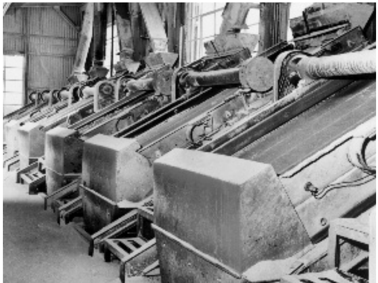
Model UP-248 vibrating screens. Proven service in the manufacture of firebrick for over 50 years.
