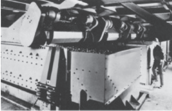
Two-deck Link-Belt® Model SS2816 dewatering screen in coal preparation plant.
