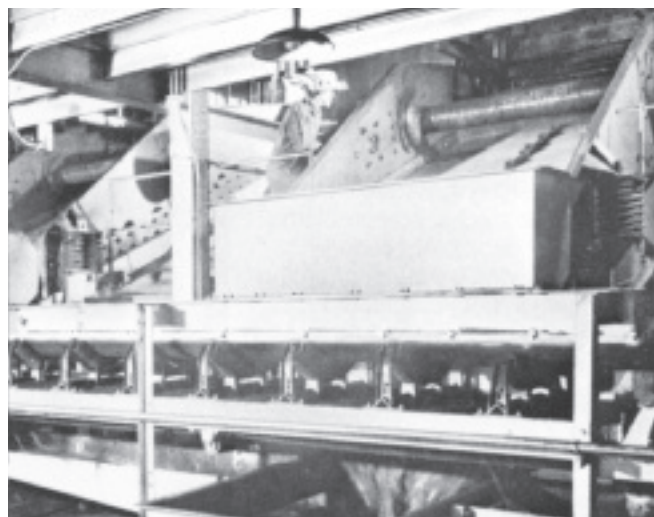
Four Link-Belt® Model Ch one-deck vibrating screens size raw coal at plus or minus 3/8". Undersize is chuted to classifiers and oversize to a belt conveyor.
