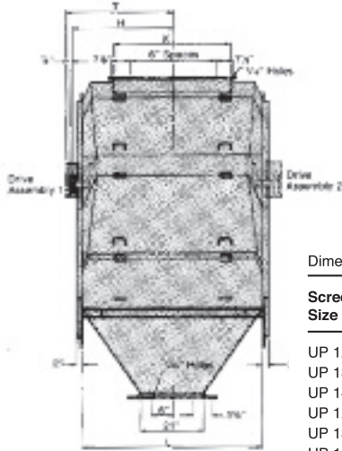
Model UP one deck, enclosed ▲
