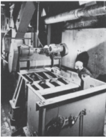
Link-Belt® Model SS2416 two-deck vibrating screen dewatering coal refuse.
