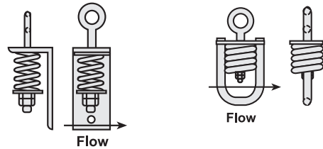
Angle Hanger
