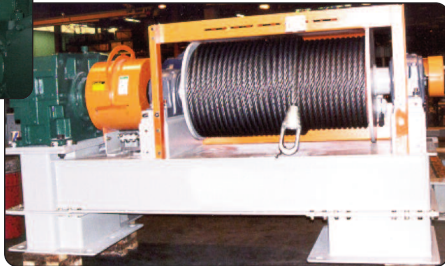
AC-Constant Tension Winch Note: Availability up to 300 hp. Line pull 1,000-100,000 lb.
