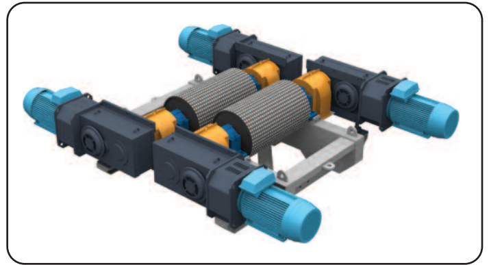
4x300HP Alignment Free Drive
