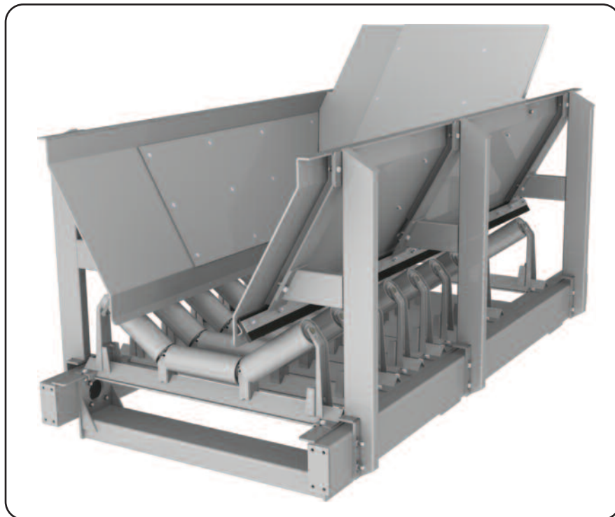
Underground Loading Section with F5000 Impact Idlers 3500 tph, 60-inch Belt Width
