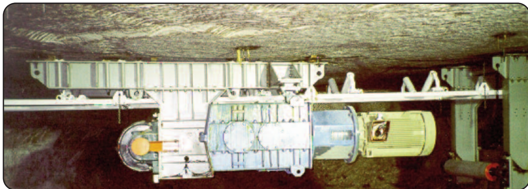
Roof-Mount 2-Pulley Alignment-Free Drive
