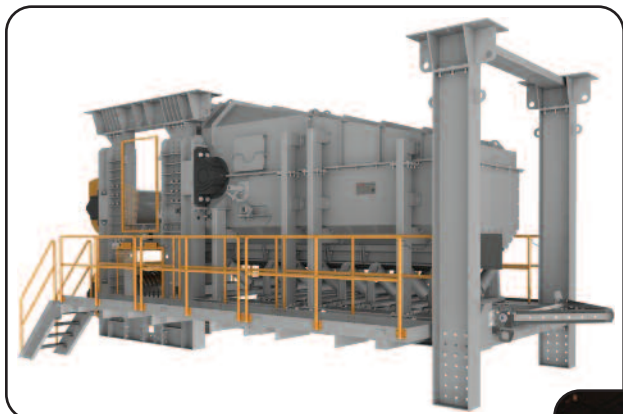
3-D Engineered Model
