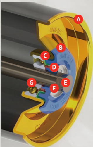
CEMA SERIES C2000 IDLER
